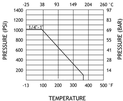
PRESSURE-TEMPERATURE RATING
